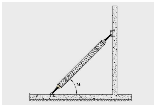
A - Angle of raking shore
