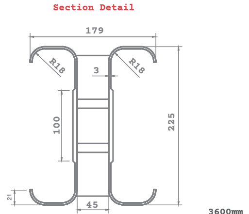
SHORE PROP 100 SECTION SIZES
