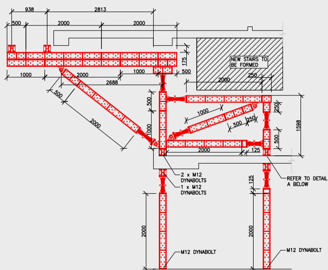
SHORE PROP 400 FRAME TYPE 1 (1 OFF)
